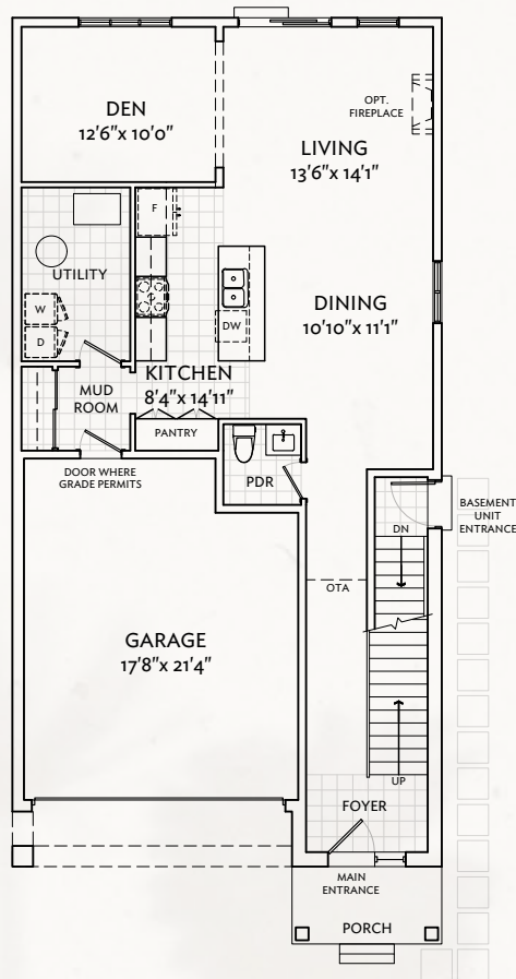
Main Floor
